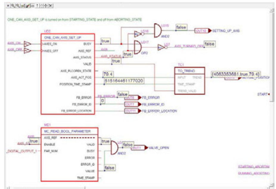
Graphical Debugger
