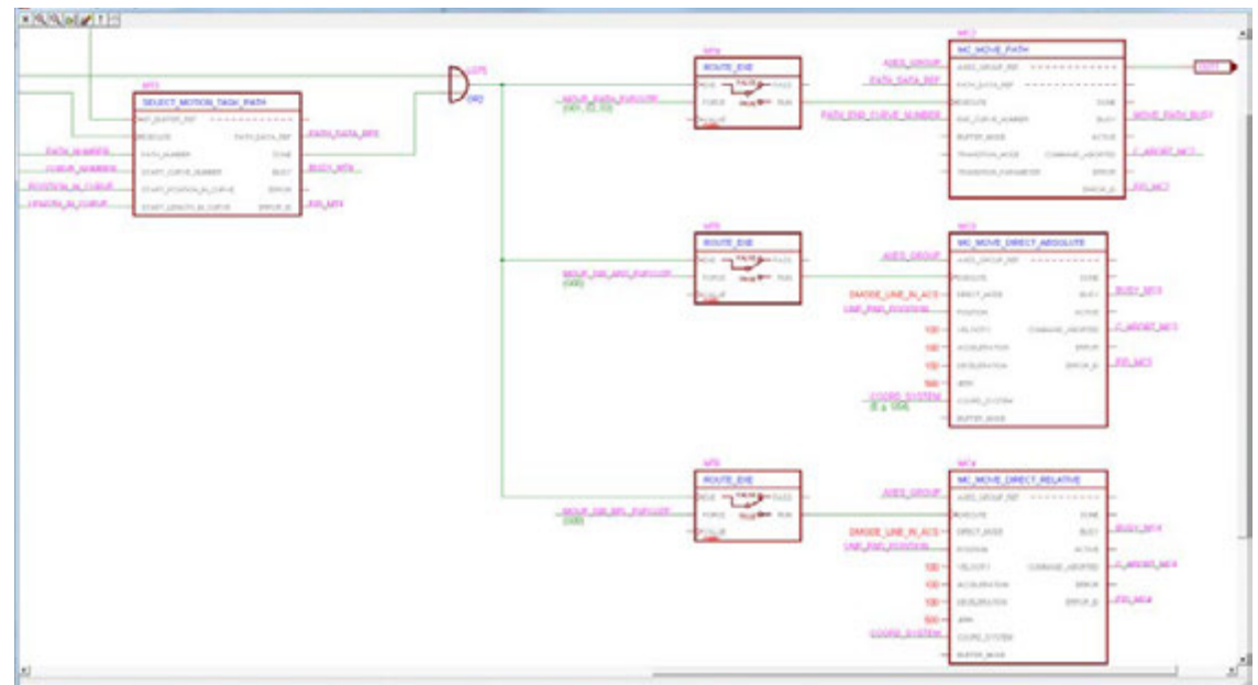
FBD Editor
